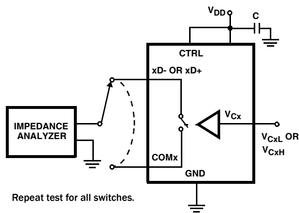
FIGURE 6. CAPACITANCE TEST CIRCUIT
