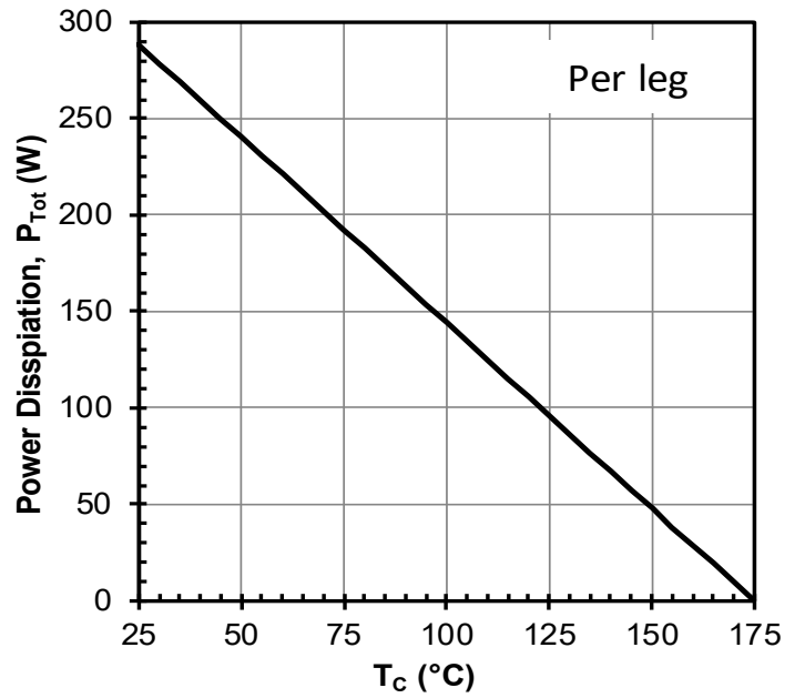
Figure 4. Power dissipation
