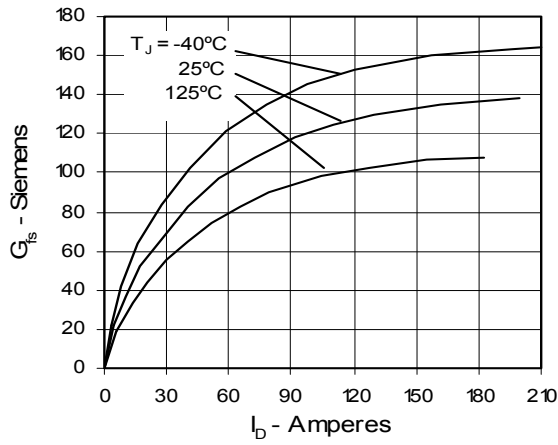
Fig. 7. Transconductance
