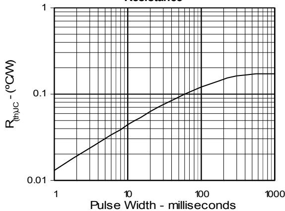
Fig. 11. Maximum Transient Thermal Resistance
