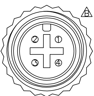
Conn.1&2 Pin Assignments Front View
