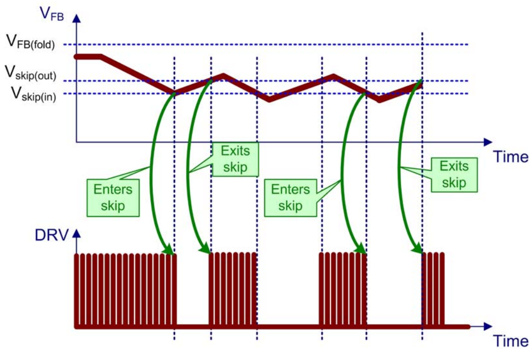
Figure 61. Skip Mode Timing Diagram
