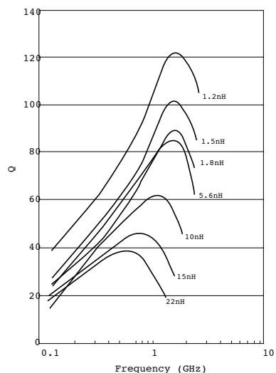
Typical Q vs. Frequency L0805
