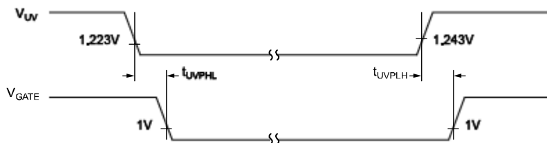
Figure 4. MIC2589/MIC2589R Undervoltage Response
