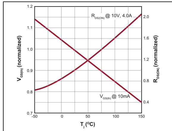
FIGURE 2-5: V_{GS} and R_{DS} Variation with Temperature.
