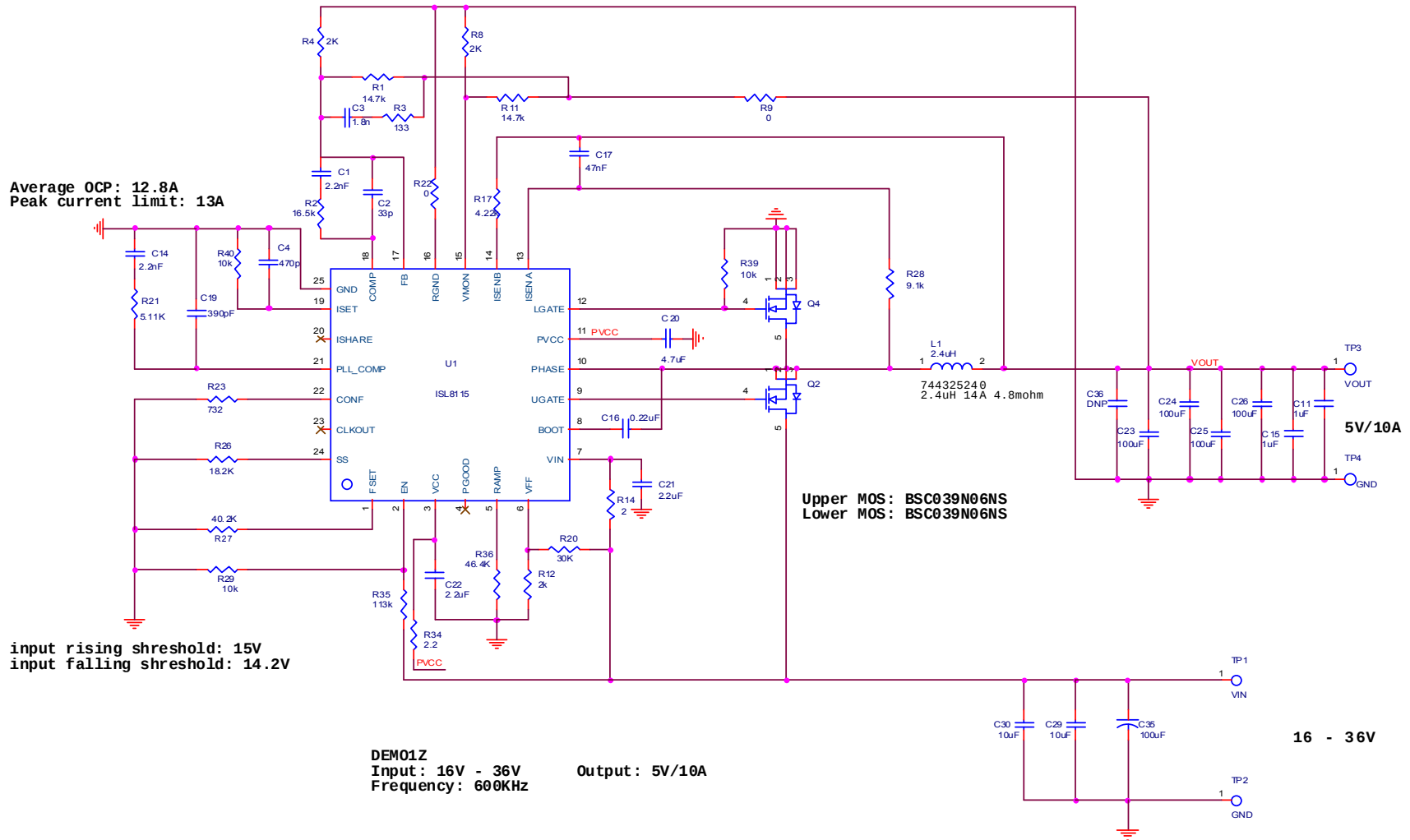
FIGURE 21. ISL8115DEMO1Z SCHEMATIC
