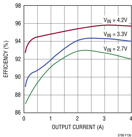
Figure 13. Low I_Q Lithium-Ion to 5V/4A Boost Converter
