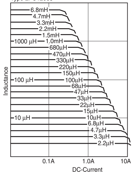
Type LPC12065
