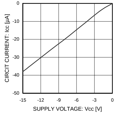
Fig. 9 Back Current
