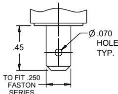
TERM. STYLES 3
