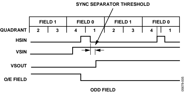
Figure 5. VSYNC Filter—Odd
