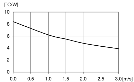
Thermal resistance vs. airspeed measured at the converter. Tested in wind tunnel with airflow and test conditions as per the Thermal consideration section. V_i = 53\text{ V} .
