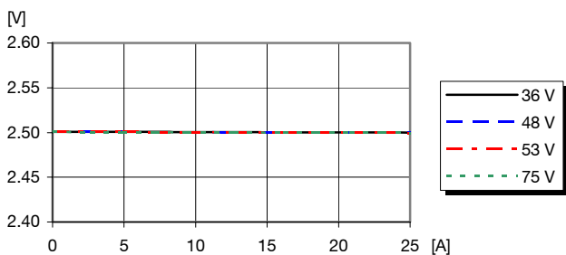
Output voltage vs. load current at T_{ref} = +25^{\circ}\text{C}
