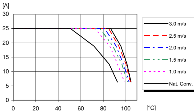
Available load current vs. ambient air temperature and airflow at V_i = 53\text{ V} . See Thermal Consideration section.
