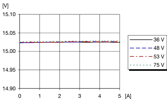
Output voltage vs. load current at T_{ref} = +25^{\circ}\text{C}
