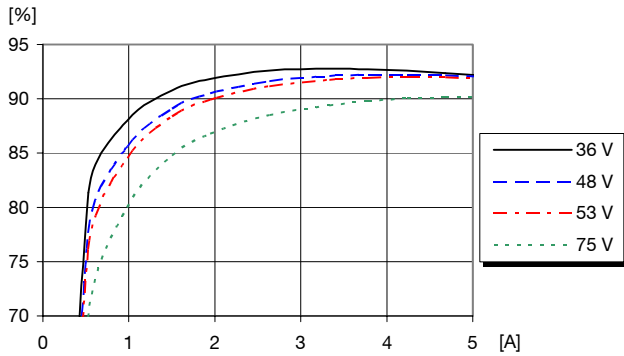
Efficiency vs. load current and input voltage at T_{ref} = +25^{\circ}\text{C}
