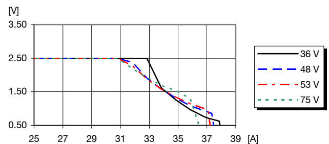
Output voltage vs. load current at I_o > \max I_o , T_{ref} = +25^{\circ}\text{C}
