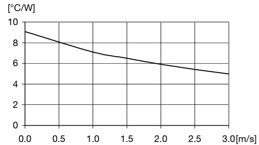
Thermal resistance vs. airspeed measured at the converter. Tested in wind tunnel with airflow and test conditions as per the Thermal consideration section. V_i = 53\text{ V} .
