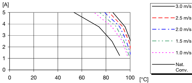
Available load current vs. ambient air temperature and airflow at V_i = 53\text{ V} . See Thermal Consideration section.
