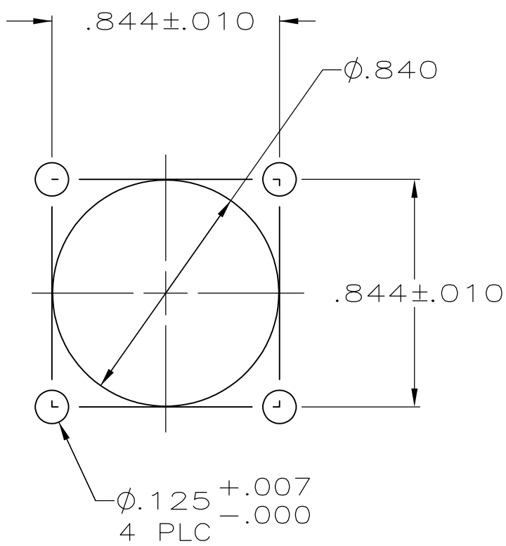
RECOMMENDED PANEL CUTOUT SCALE 2:1
