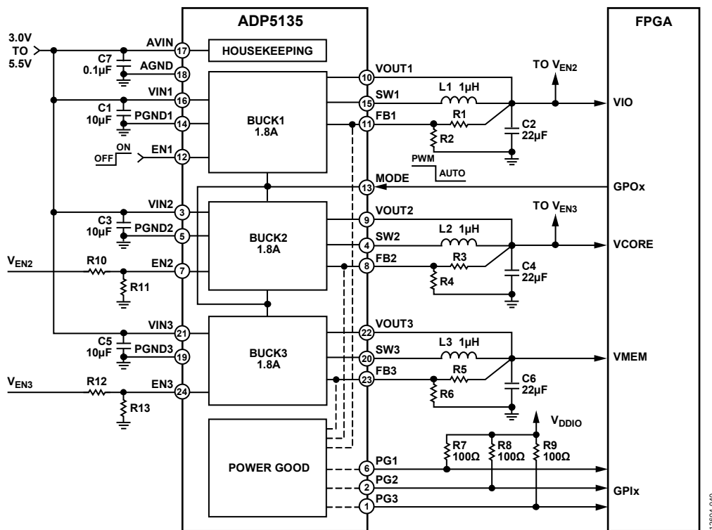
Figure 40. ADP5135 Adjustable Output Voltages with Precision Enable Pins
