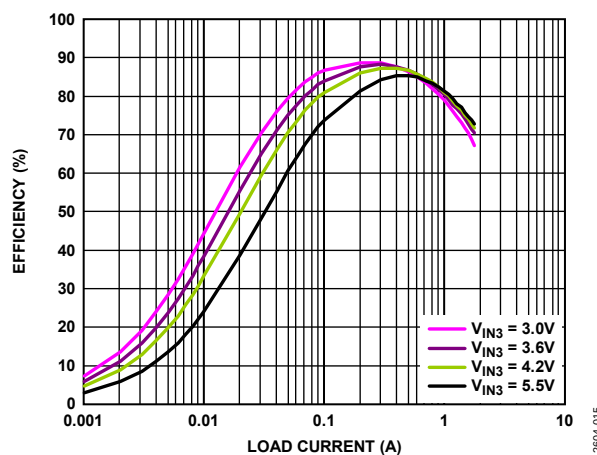
Figure 15. BUCK3 Efficiency vs. Load Current, Across Input Voltage, V_{OUT3} = 1.2\text{ V} , PWM Mode
