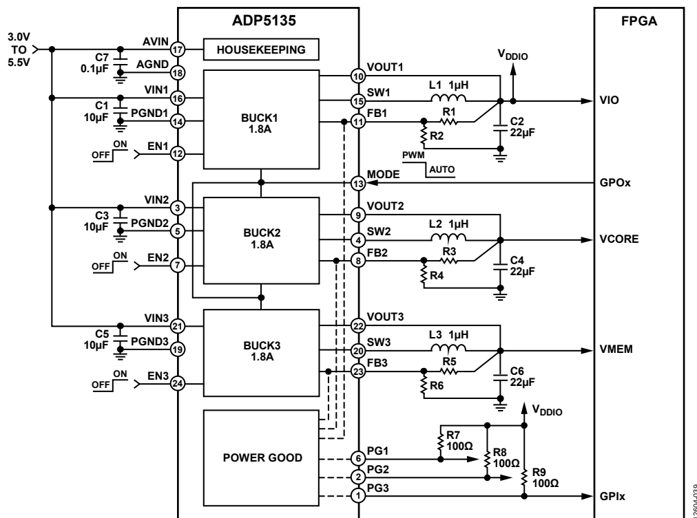
Figure 39. Processor System Power Management with PSM/PWM Control and Power Good
