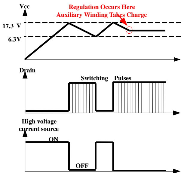
Figure 3: VCC UVLO
