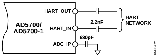
Figure 22. AD5700/AD5700-1 Using Internal Filter on HART_IN
