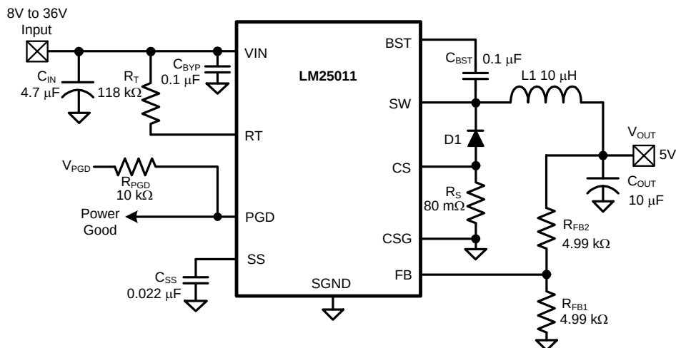
Figure 21. Example Circuit
