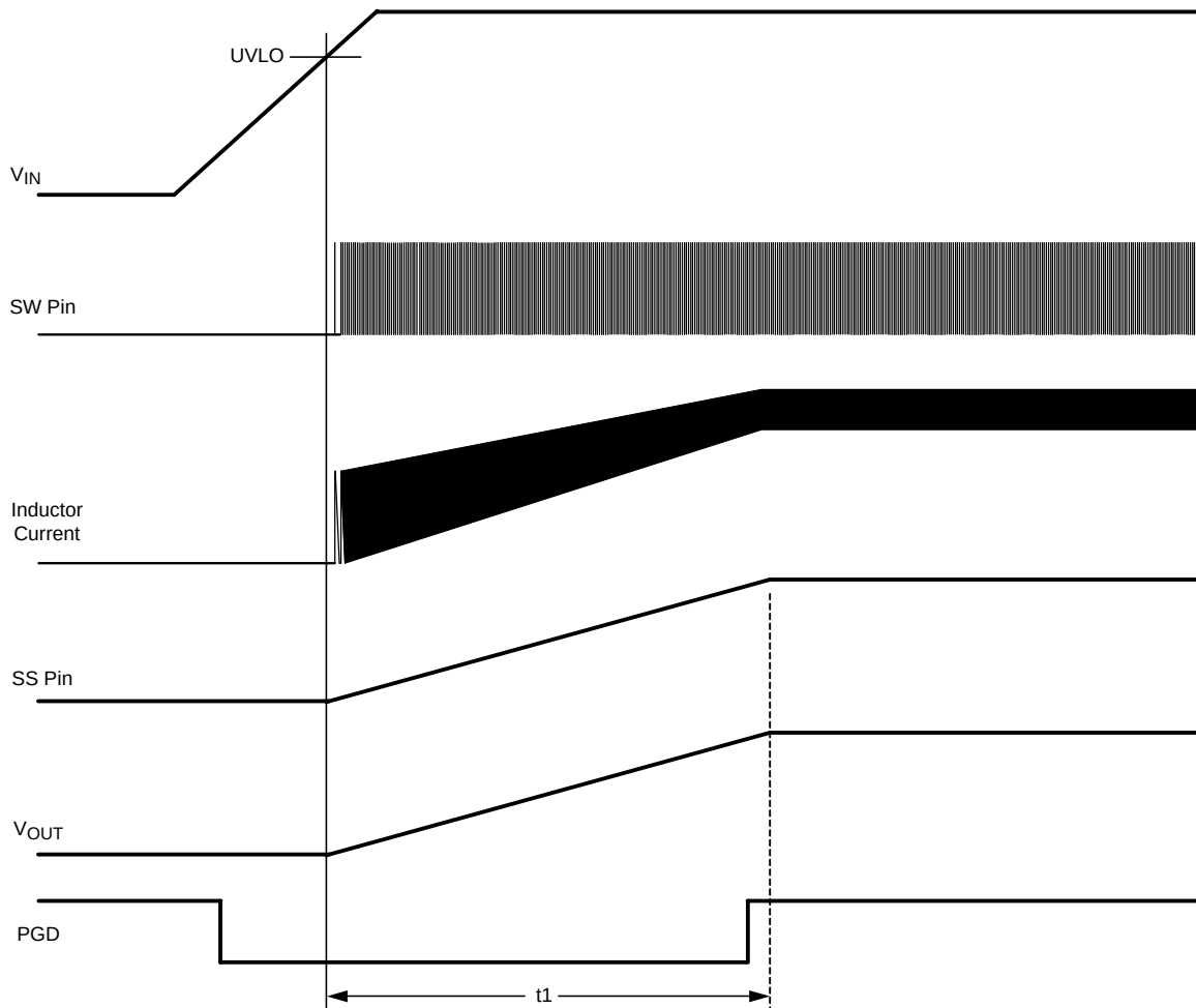
Figure 17. Startup Sequence
