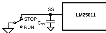
Figure 20. Shutdown Implementation
