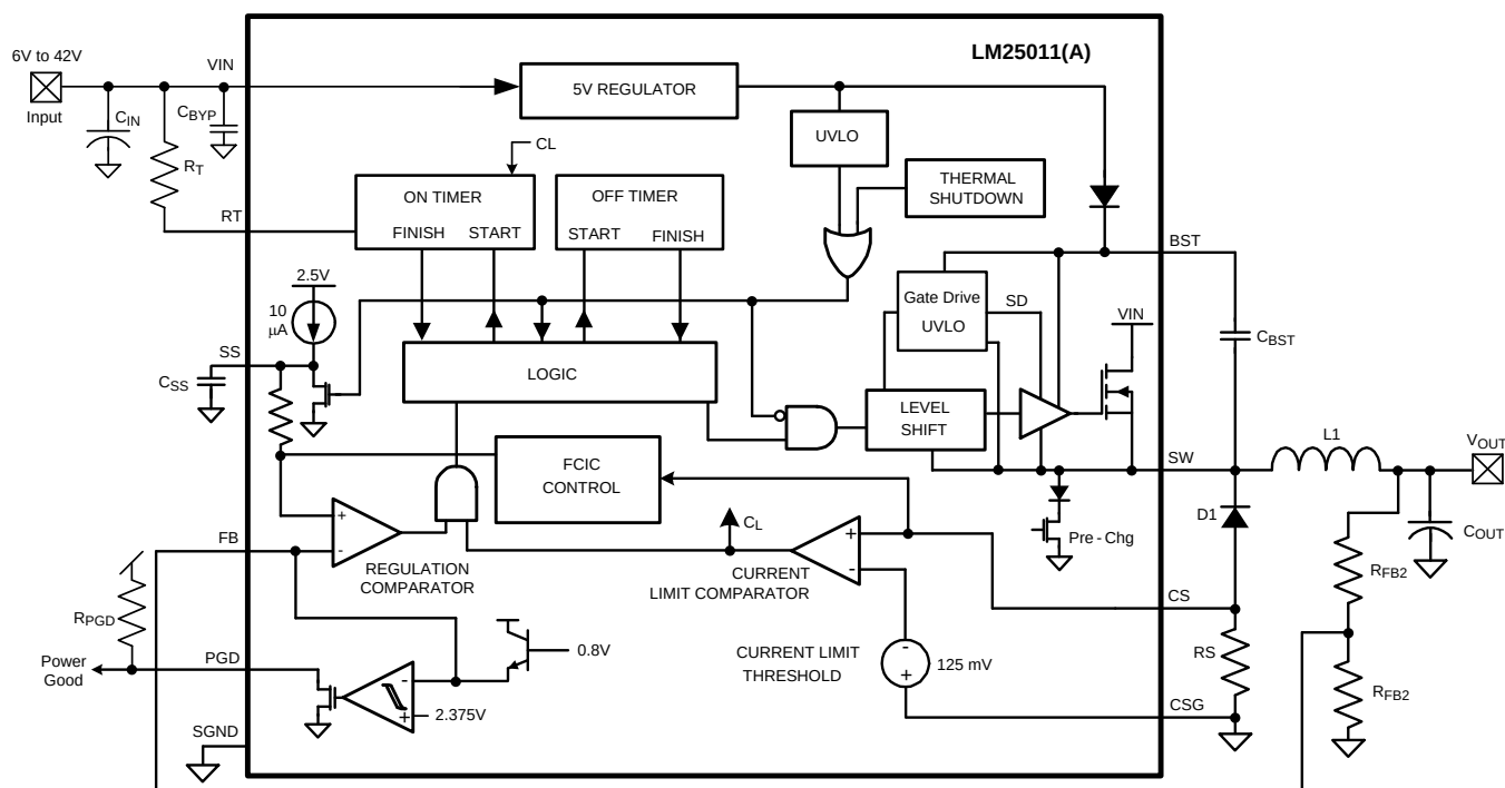
Figure 16. Block Diagram
