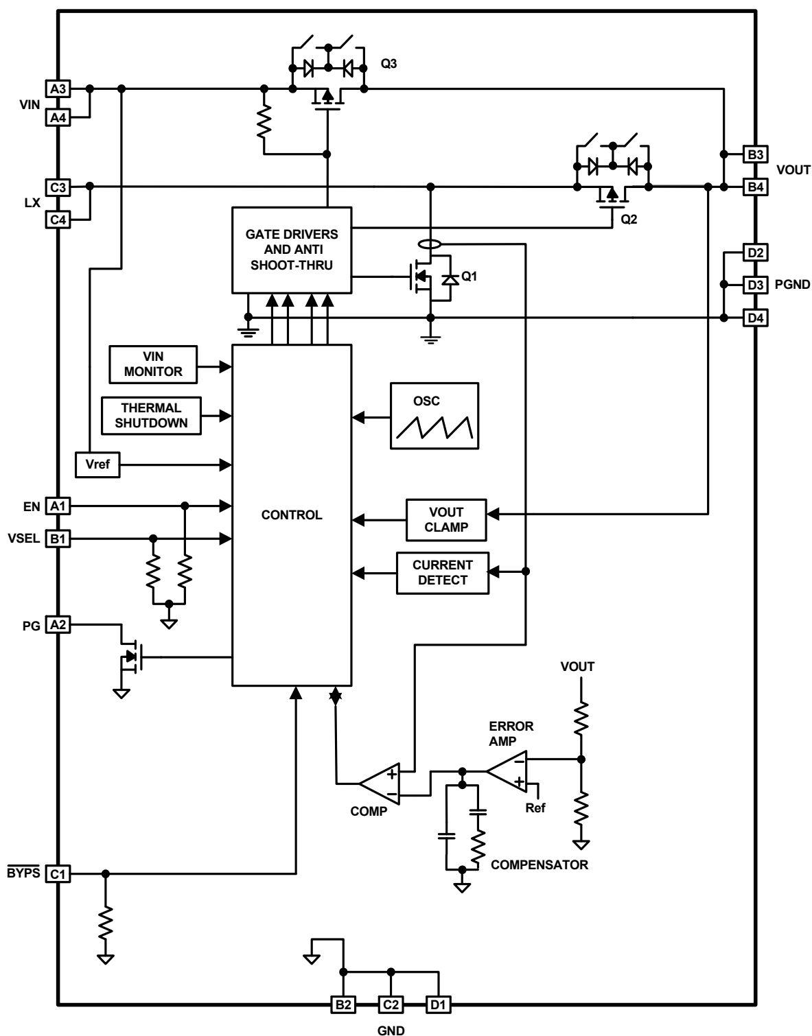
FIGURE 3. BLOCK DIAGRAM
