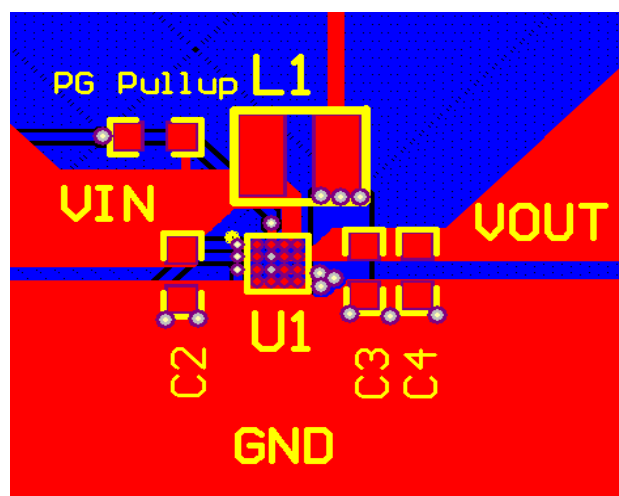
FIGURE 22. LAYOUT RECOMMENDATION
