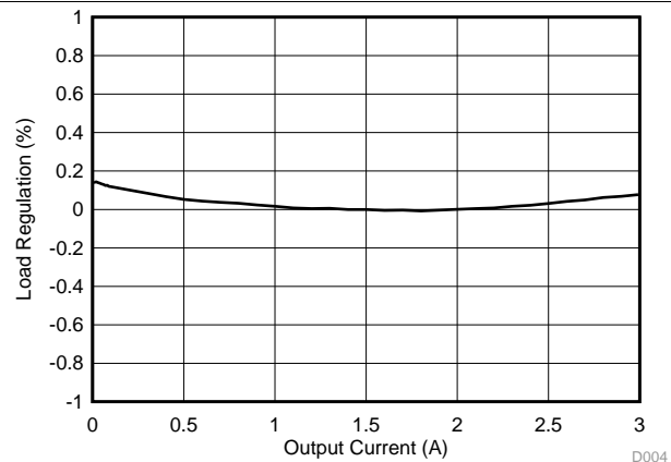
Figure 34. TPS563219 Load Regulation, V_I = 12\text{ V}
