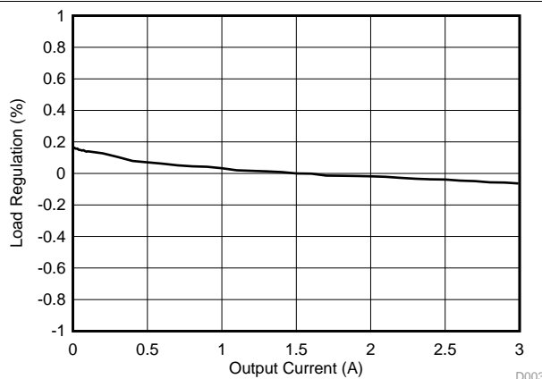
Figure 33. TPS563219 Load Regulation, V_I = 5\text{ V}
