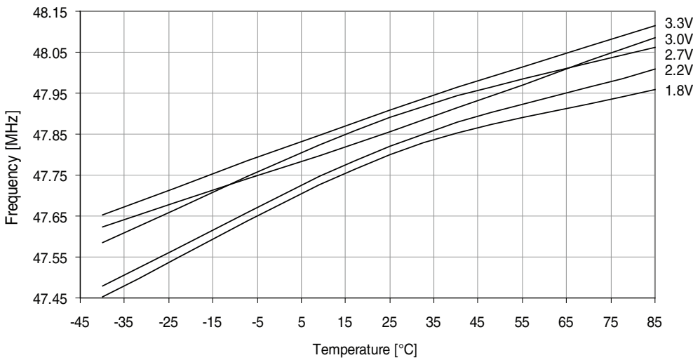
Figure 37-245. 48MHz internal oscillator frequency vs. temperature. DFLL enabled, from the 32.768kHz internal oscillator.
