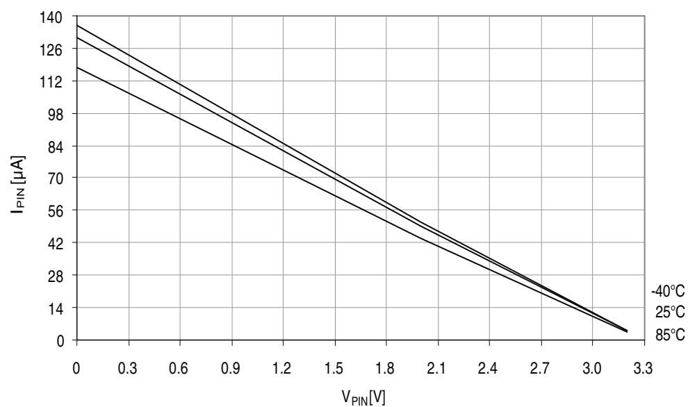
Figure 37-313. Reset pin pull-up resistor current vs. reset pin voltage.
