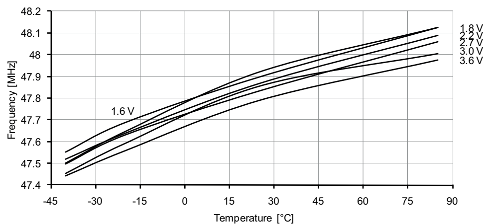
Figure 37-162. 48MHz internal oscillator frequency vs. temperature.
