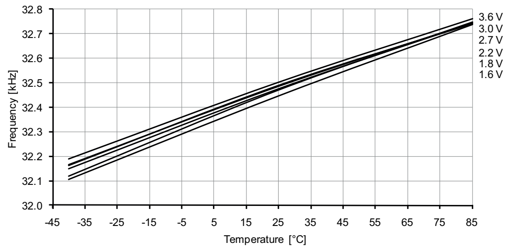
Figure 37-69. 32.768kHz internal oscillator frequency vs. temperature.
