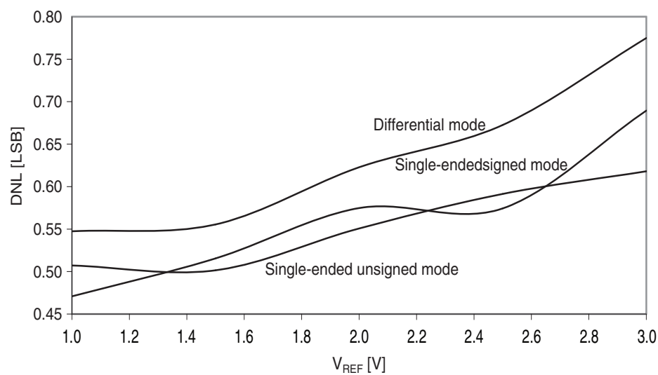
Figure 37-287. DNL error vs. external V_{REF} . T = 25\text{ }^{\circ}\text{C} , V_{CC} = 3.6\text{V} , external reference.
