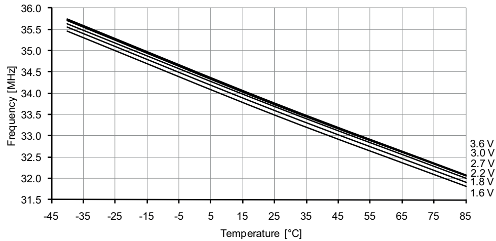
Figure 37-75. 32MHz internal oscillator frequency vs. temperature. DFLL enabled, from the 32.768kHz internal oscillator.
