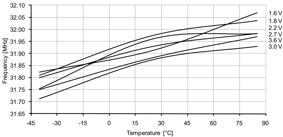
Figure 37-158. 32MHz internal oscillator frequency vs. temperature. DFLL enabled, from the 32.768kHz internal oscillator.
