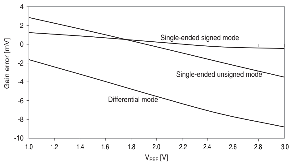
Figure 37-290. Gain error vs. V_{REF} .
