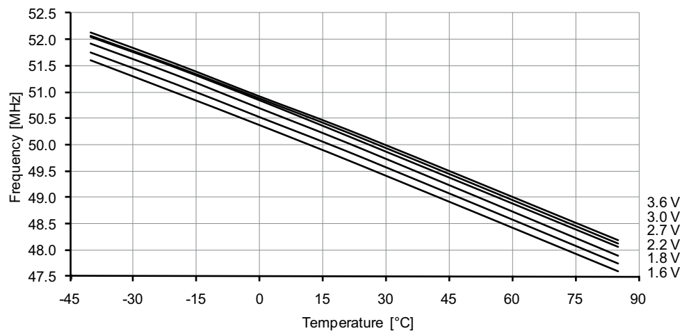
Figure 37-162. 48MHz internal oscillator frequency vs. temperature.
