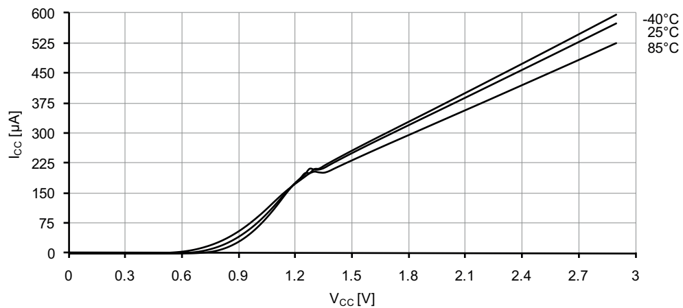
Figure 37-67. Power-on reset current consumption vs. V_{CC} .
