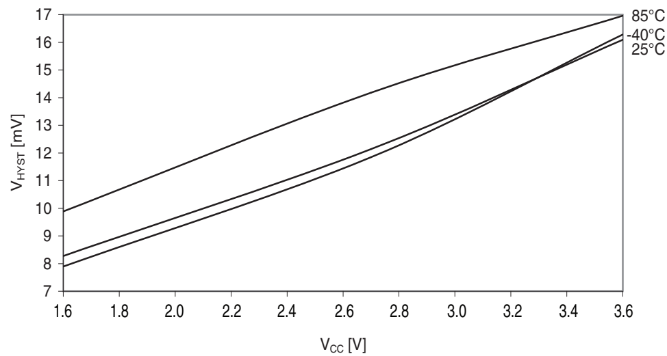
Figure 37-217. Analog comparator hysteresis vs. V_{CC} . High-speed, small hysteresis.
