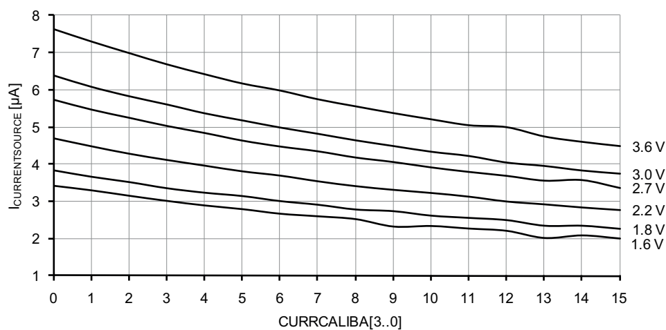
Figure 37-56. Analog comparator current source vs. calibration value.
