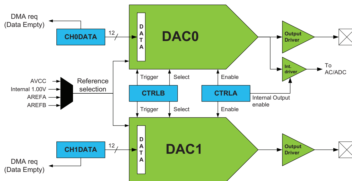
Figure 29-1. DAC overview.
