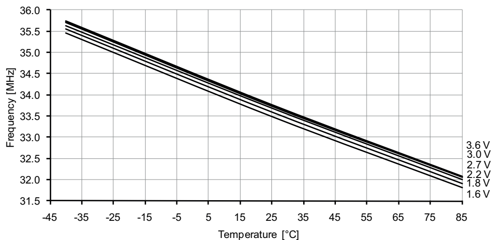
Figure 37-75. 32MHz internal oscillator frequency vs. temperature.
