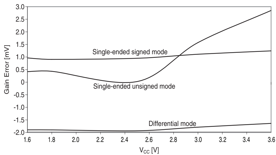
Figure 37-291. Gain error vs. V_{CC} .
