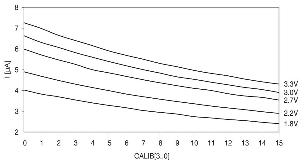
Figure 37-304. Analog comparator current source vs. calibration value.
