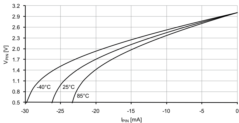
Figure 37-24. I/O pin output voltage vs. source current.
