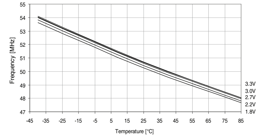
Figure 37-327. 48MHz internal oscillator frequency vs. temperature. DFLL disabled.
