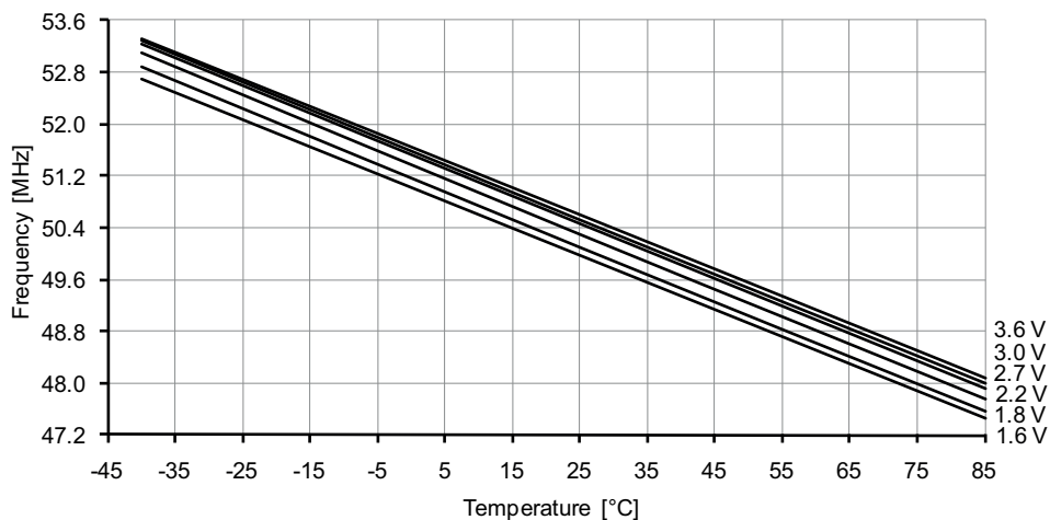
Figure 37-78. 48MHz internal oscillator frequency vs. temperature. DPLL disabled.
