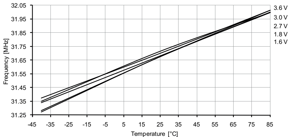
Figure 37-75. 32MHz internal oscillator frequency vs. temperature.
