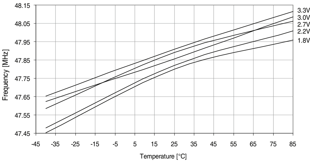
Figure 37-328. 48MHz internal oscillator frequency vs. temperature. DFLL enabled, from the 32.768kHz internal oscillator.
