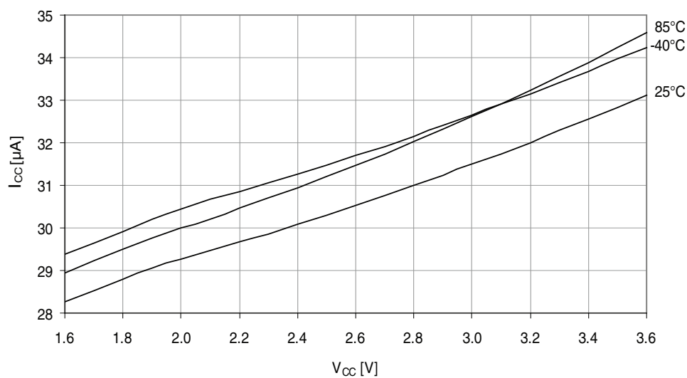
Figure 37-259. Idle mode supply current vs. V_{\text{CC}} .
