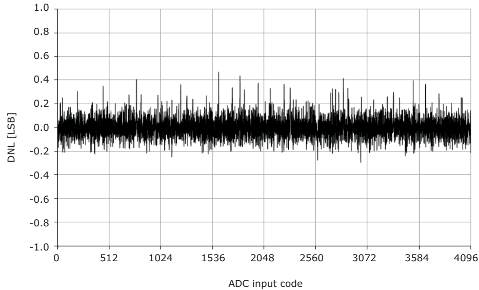
Figure 37-40. DNL error vs. input code.
