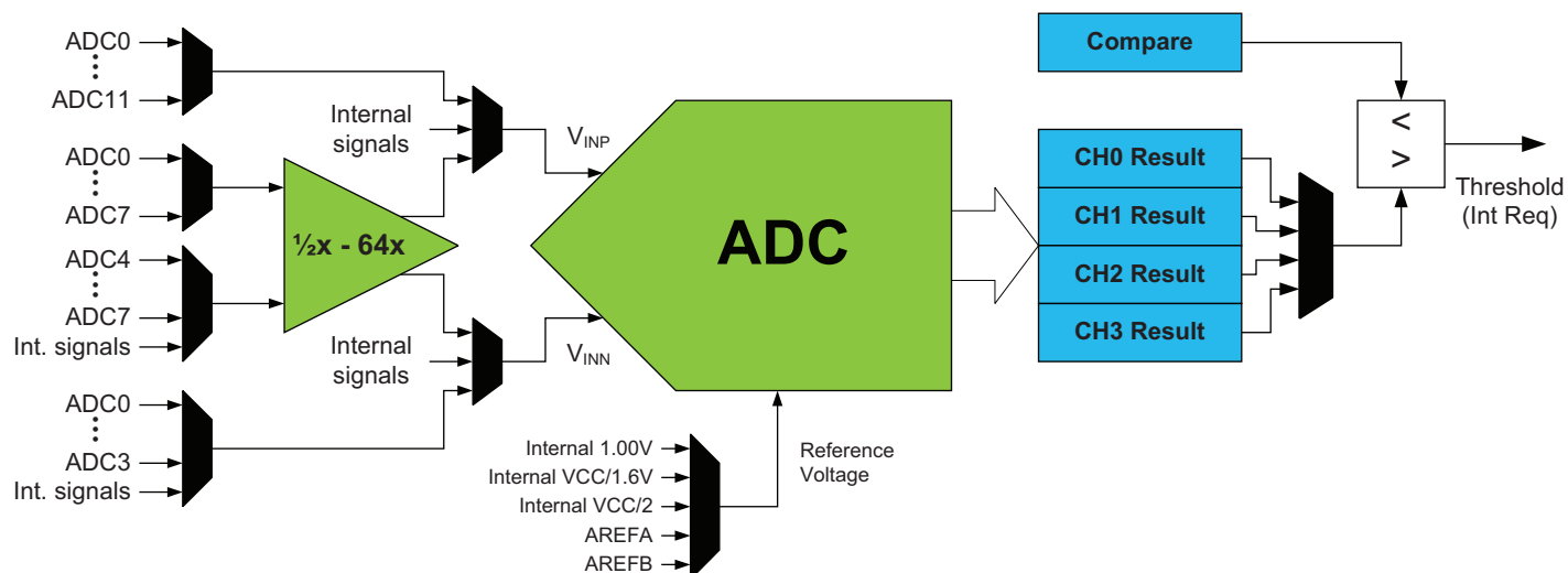
Figure 28-1. ADC overview.
