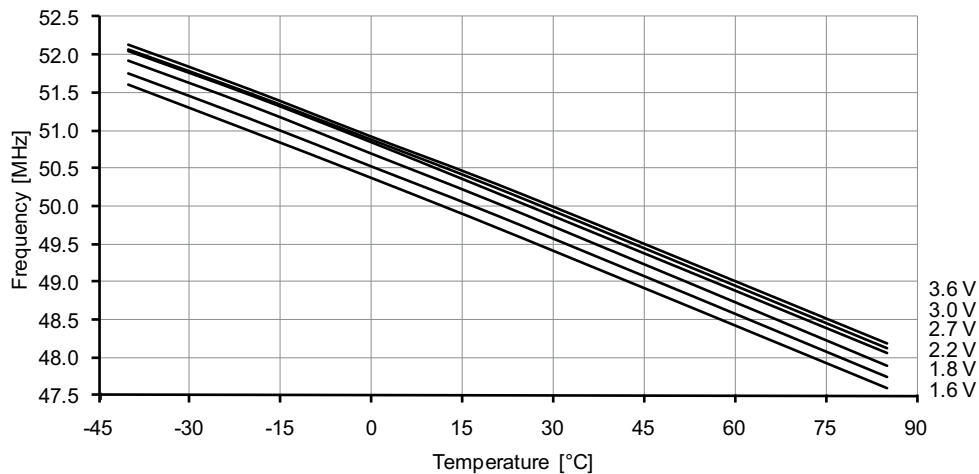
Figure 37-161. 48MHz internal oscillator frequency vs. temperature. DFLL disabled.
