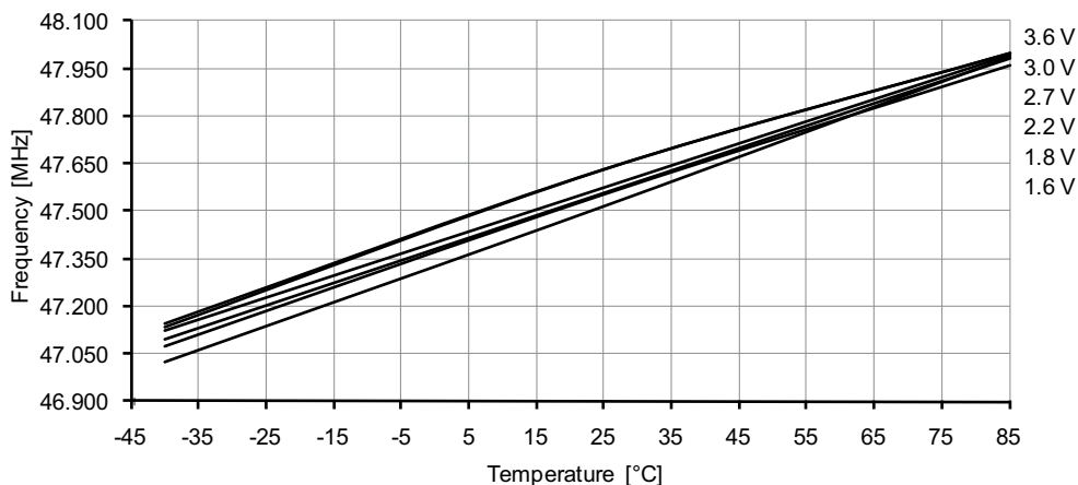
Figure 37-79. 48MHz internal oscillator frequency vs. temperature. DPLL enabled, from the 32.768kHz internal oscillator.
