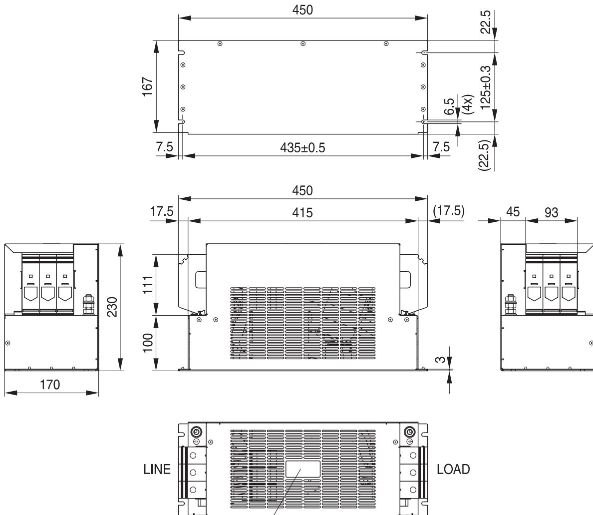
Marking Dimensional drawing
