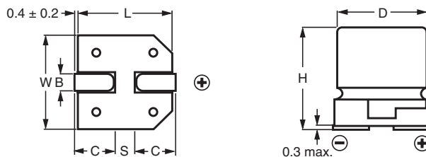
Fig.2 Dimensional outline
