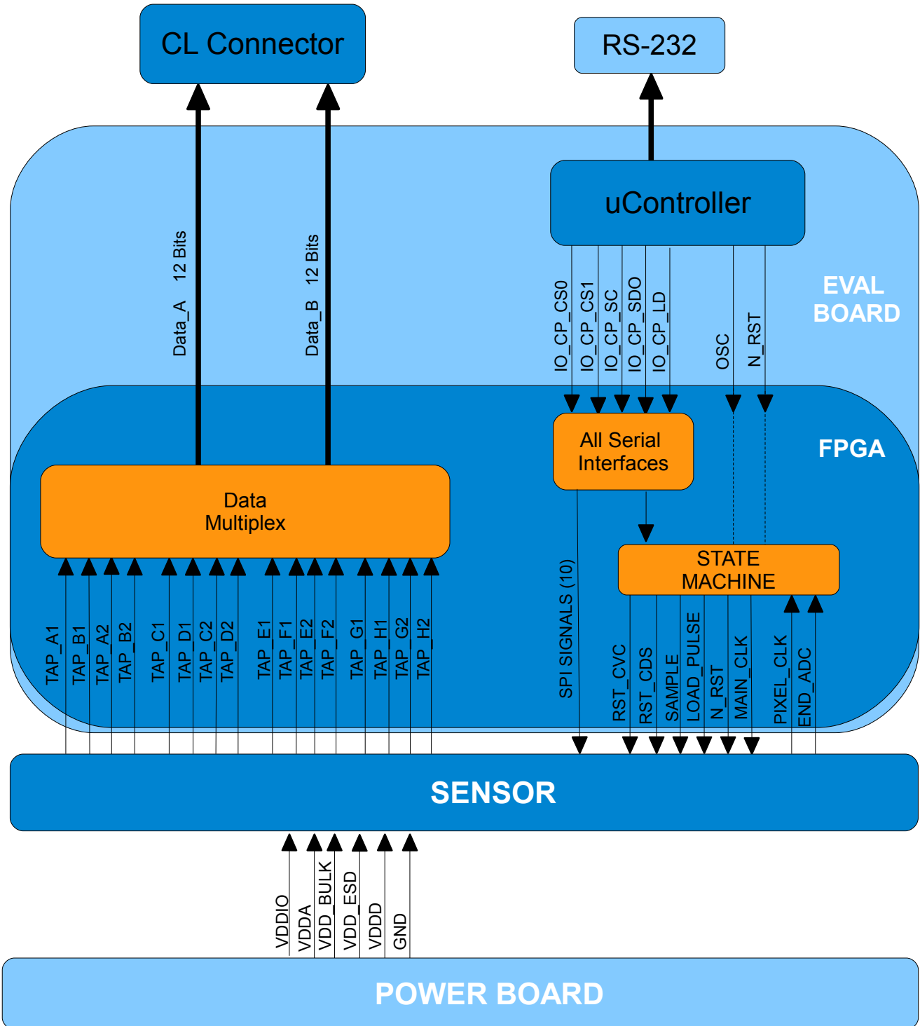
Figure 1: Block Diagram
