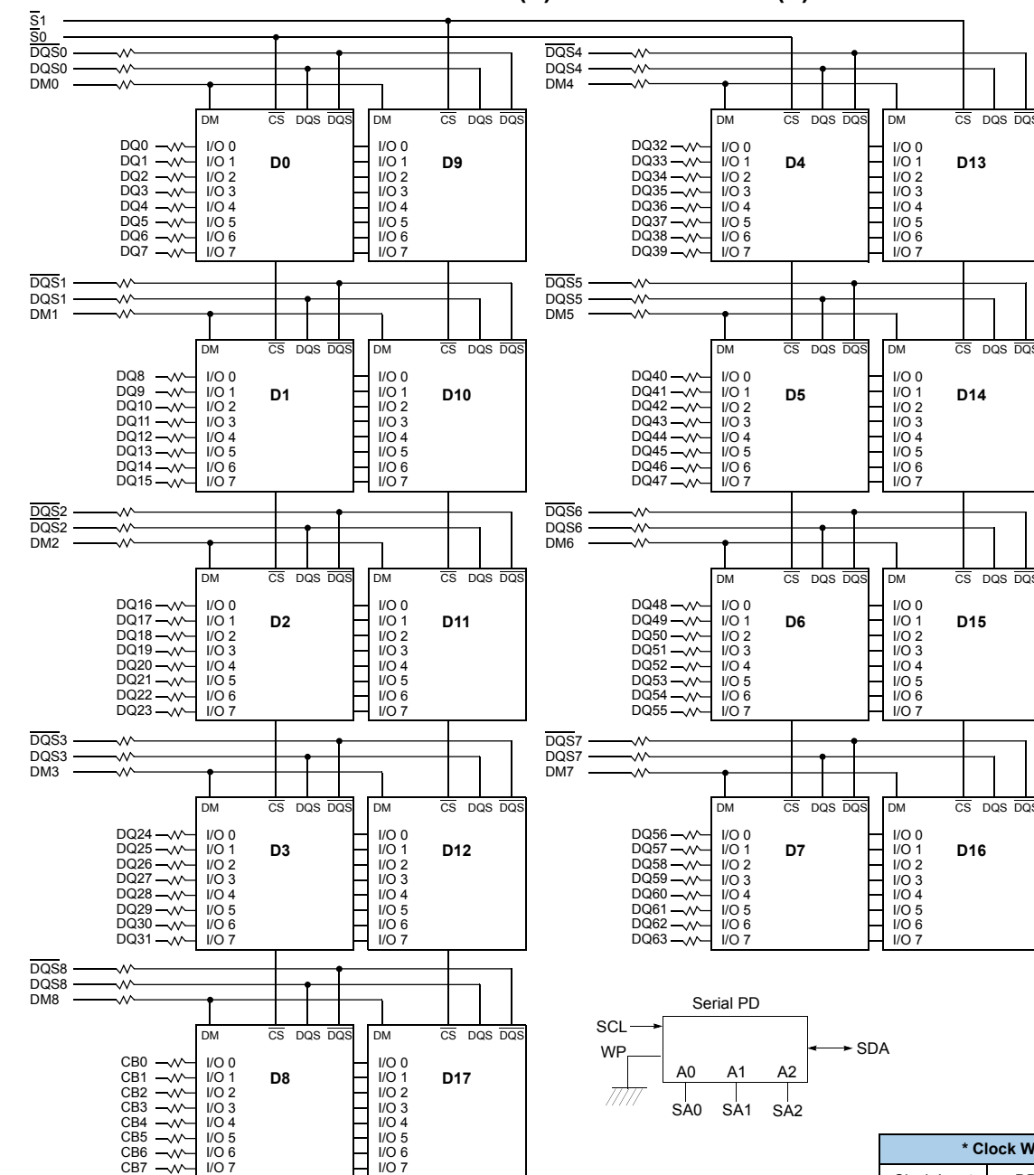
Functional Block Diagram: 512MB, 64Mx72 ECC Module (Populated as 2 ranks of x8 DDR2 SDRAMs) M391T6453FG(Z)3 / M391T6453FG(Z)0
