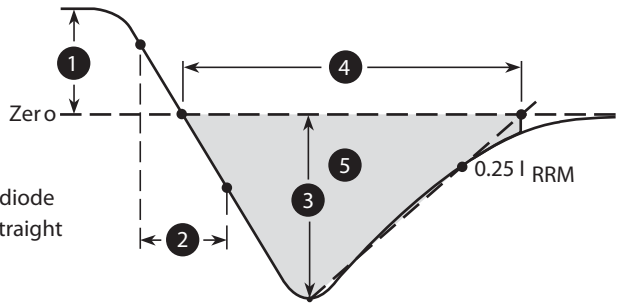
Figure 10, Diode Reverse Recovery Waveform and Definition
