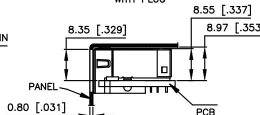
SECTION B-B SIDE VIEW SHOWING WITH PANEL AND PCB
