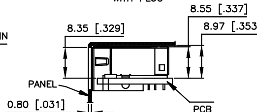
SECTION B-B SIDE VIEW SHOWING WITH PANEL AND PCB
