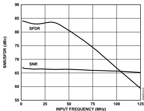
Figure 27. AD9237-65 SNR/SFDR vs. Input Frequency
