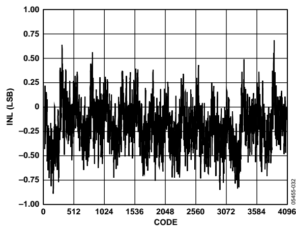
Figure 28. Typical INL
