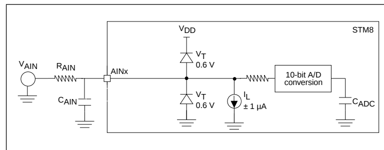
Figure 44: Typical application with ADC
