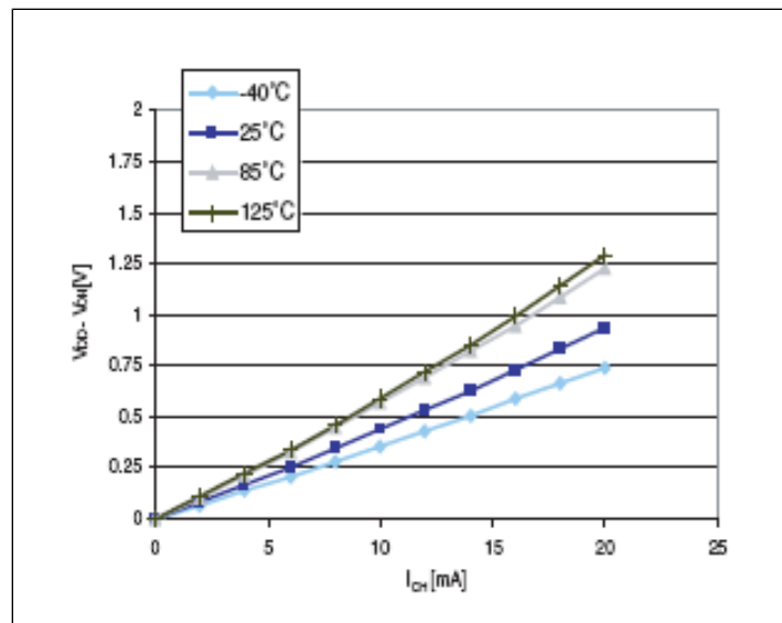
Figure 33: Typ. V_{DD} - V_{OH} @ V_{DD} = 5\text{ V} (high sink ports)
