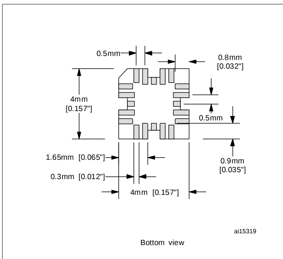
Figure 50: Recommended footprint for on-board emulation
