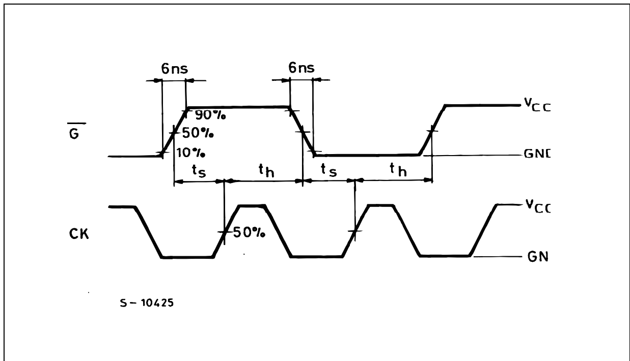
WAVEFORM 3 : SETUP AND HOLD TIME ( \overline{G} TO CK) (f=1MHz; 50% duty cycle)
