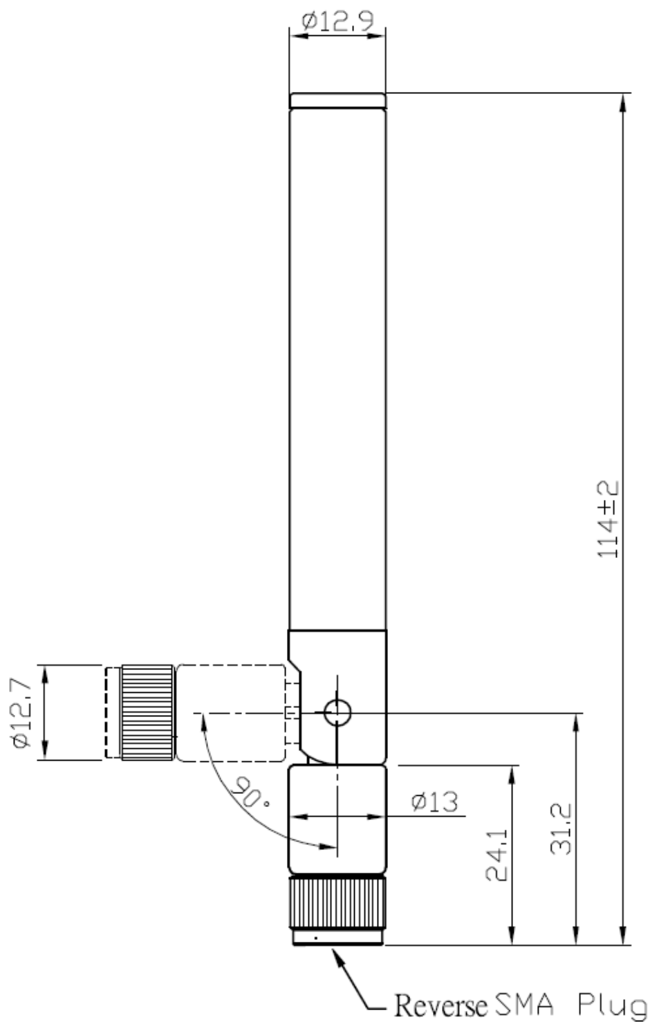
Figure 1 Physical Dimensions
