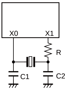
Example oscillation circuit
