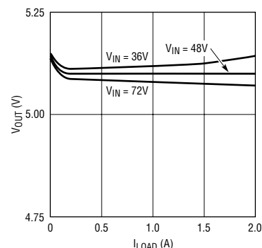
Output Load Regulation
