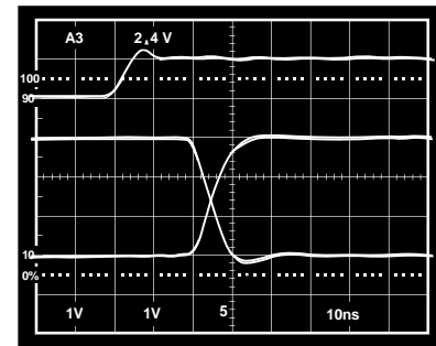
Figure 13. RS-422 Driver; R_{L\text{DIFF}} = 100\text{ }\Omega , C_{L1} = C_{L2} = 100\text{ pF}
