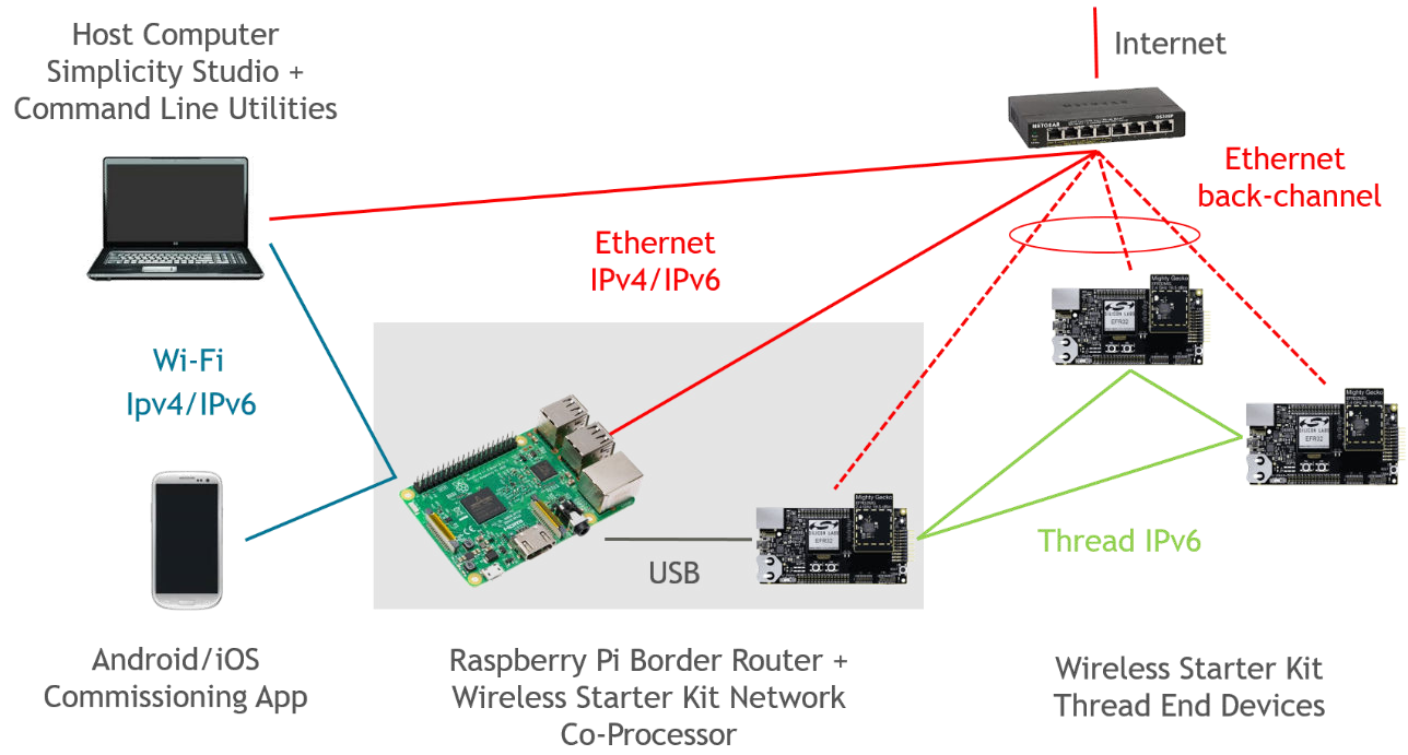
Figure 1.1. Thread System Components
