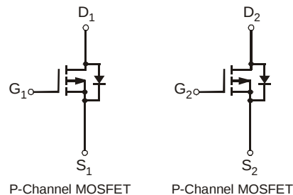
SOP-8L
