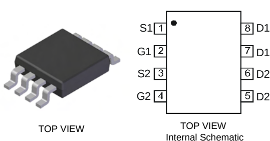
SOP-8L
