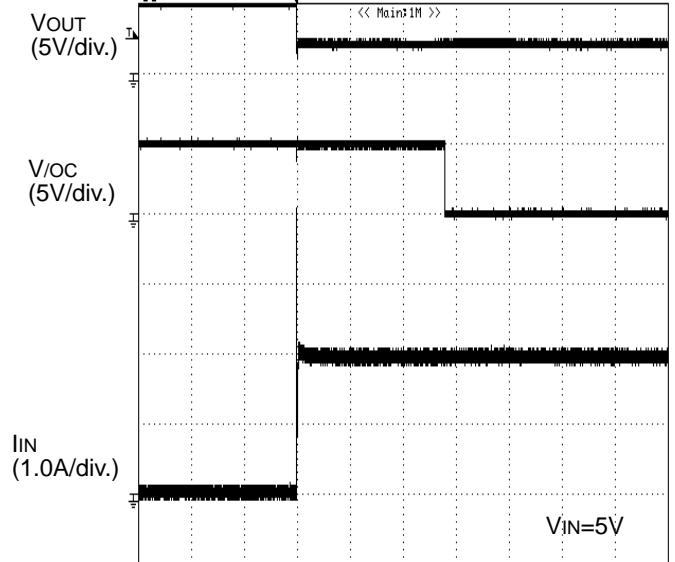
Figure 37. Over-Current Response 1 Load Connected at Enable
