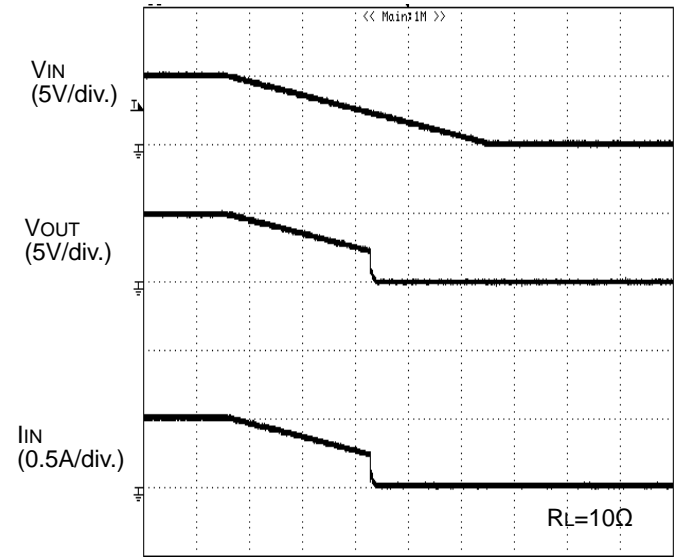
Figure 39. UVLO Response Decreasing VIN
