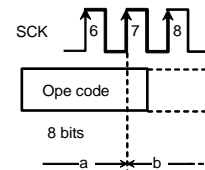
Figure 42. WREN/WRDI cancel valid timing
