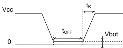
Figure 54. Rise waveform
