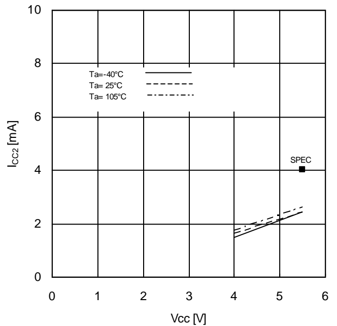
Figure 12. Supply Current (Read) vs Supply Voltage (f sck =10MHz)
