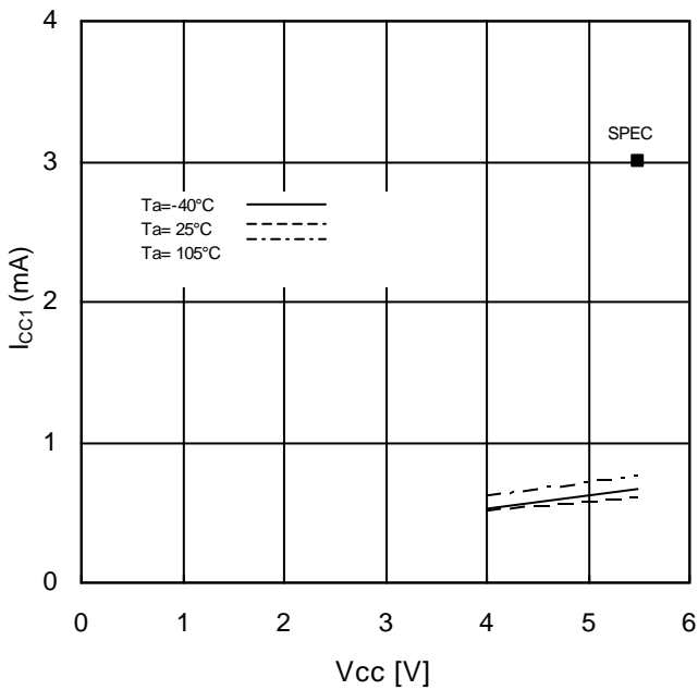
Figure 11. Supply Current (Write) vs Supply Voltage (f sck =10MHz)
