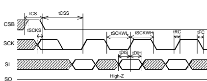
Figure 2-(a). Input timing
