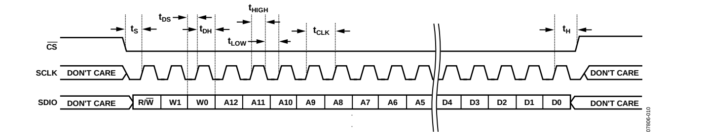
Figure 26. Serial Control Port Write—MSB First, 16-Bit Instruction, Timing Measurements
