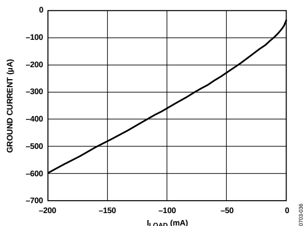
Figure 38. Ground Current vs. Load Current ( I_{LOAD} ), V_{OUT} = -1.22\text{ V}
