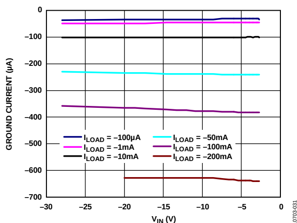
Figure 33. Ground Current vs. Input Voltage ( V_{IN} ), V_{OUT} = -1.8\text{ V}
