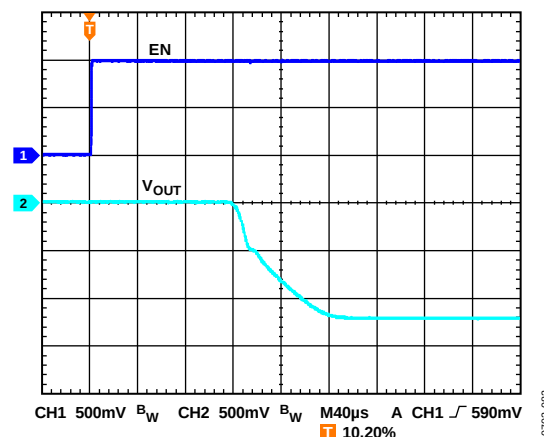
Figure 84. Typical Start-Up Behavior, Positive Going Enable
