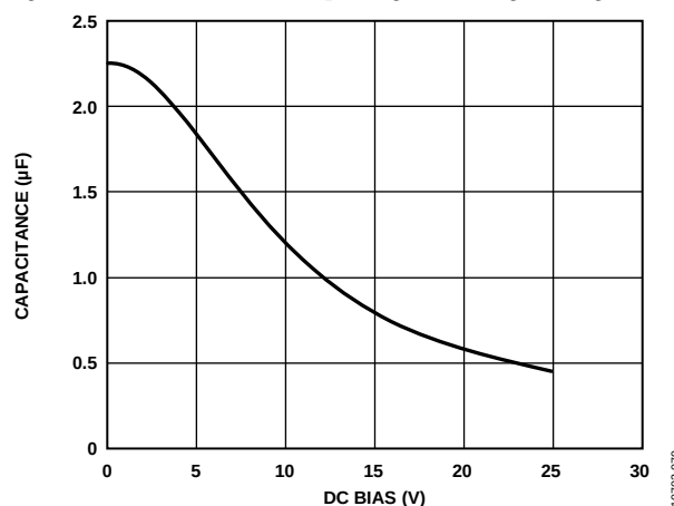
Figure 81. Capacitance vs. DC Bias Characteristics
