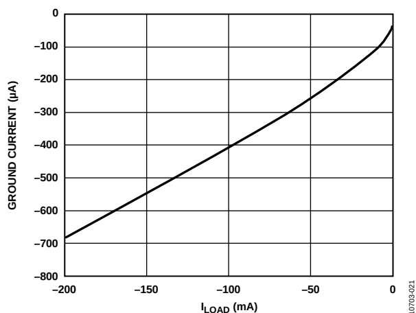
Figure 23. Ground Current vs. Load Current ( I_{LOAD} ), V_{OUT} = -5\text{ V}
