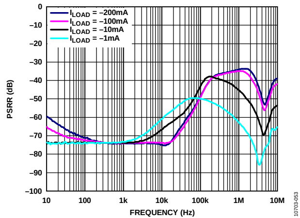
Figure 55. Power Supply Rejection Ratio (PSRR) vs. Frequency, V_{OUT} = -3\text{ V} vs. Different Load Currents ( I_{LOAD} ), V_{IN} = -4.0\text{ V}
