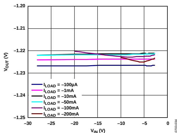
Figure 36. Output Voltage ( V_{OUT} ) vs. Input Voltage ( V_{IN} ), V_{OUT} = -1.22\text{ V}
