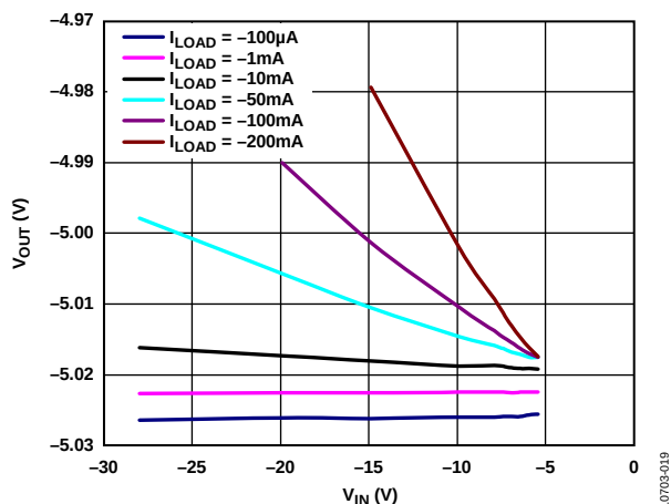
Figure 21. Output Voltage vs. Input Voltage ( V_{IN} ), V_{OUT} = -5\text{ V}
