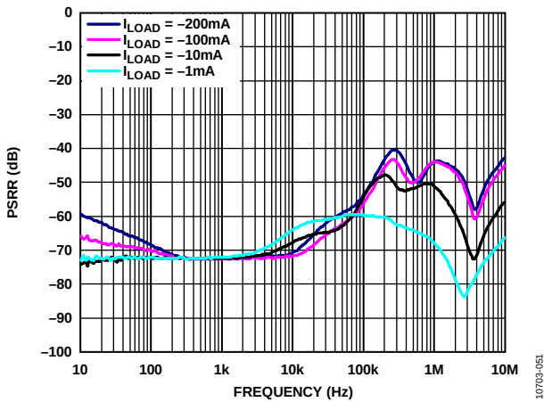
Figure 53. Power Supply Rejection Ratio (PSRR) vs. Frequency, V_{OUT} = -1.8\text{ V} vs. Different Load Currents ( I_{LOAD} ), V_{IN} = -5.5\text{ V}
