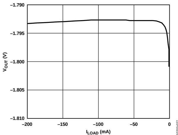
Figure 29. Output Voltage ( V_{OUT} ) vs. Load Current ( I_{LOAD} ), V_{OUT} = -1.8\text{ V}
