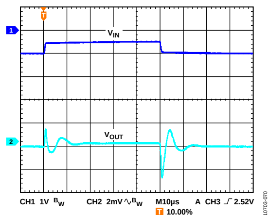
Figure 72. Line Transient Response, 500 mV Step, V_{OUT} = -15\text{ V} , Noise Reduction Network, I_{LOAD} = -10\text{ mA}
