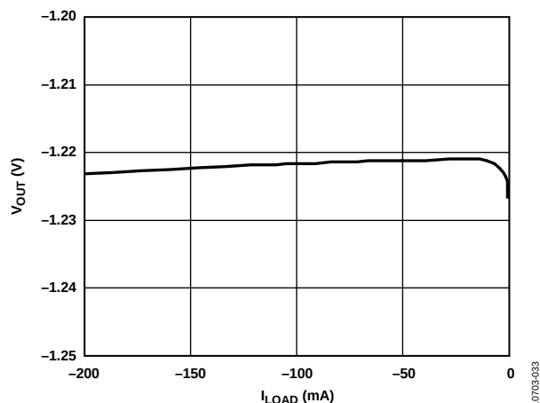
Figure 35. Output Voltage ( V_{OUT} ) vs. Load Current ( I_{LOAD} ), V_{OUT} = -1.22\text{ V}
