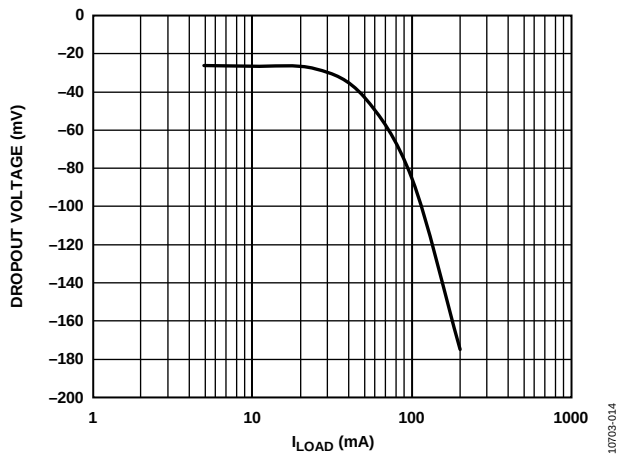
Figure 16. Dropout Voltage vs. Load Current ( I_{LOAD} )
