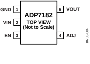
Figure 4. 5-Lead TSOT Pin Configuration, Adjustable Output Voltage
