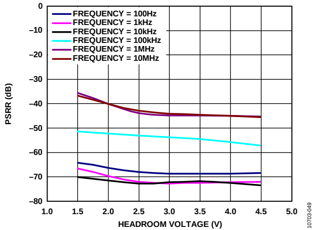
Figure 51. Power Supply Rejection Ratio (PSRR) vs. Headroom Voltage, V_{OUT} = -1.22\text{ V} , Load Current ( I_{LOAD} ) = -200\text{ mA}
