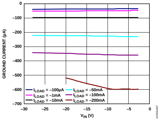
Figure 39. Ground Current vs. Input Voltage ( V_{IN} ), V_{OUT} = -1.22 V
