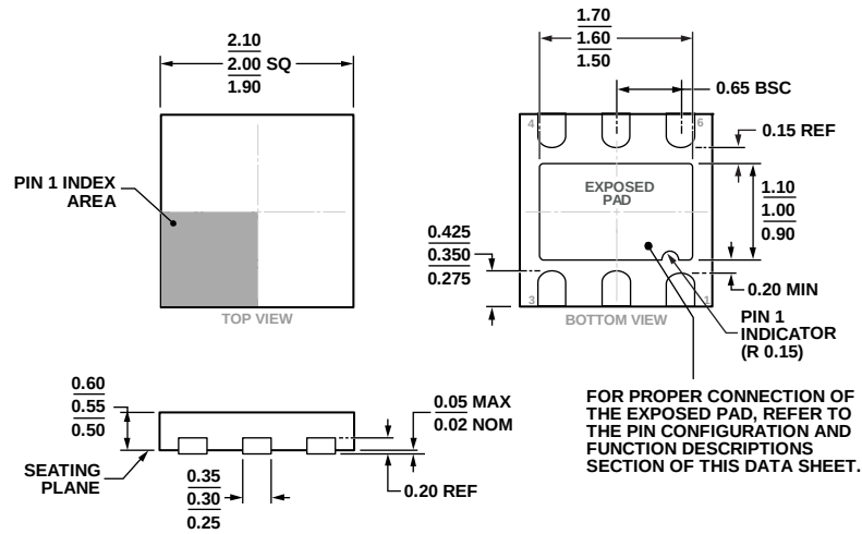
Figure 104. 6-Lead Lead Frame Chip Scale Package [LFCSP_UD] 2.00 mm × 2.00 mm Body, Ultra Thin, Dual Lead (CP-6-3) Dimensions shown in millimeters
