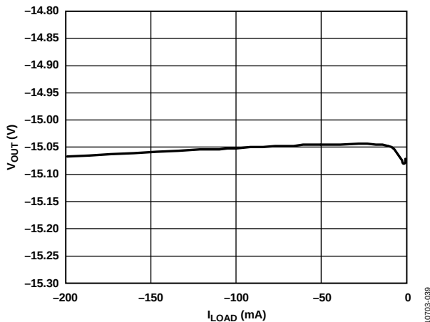
Figure 41. Output Voltage ( V_{OUT} ) vs. Load Current ( I_{LOAD} ), Adjustable Output Voltage, V_{OUT} = -15 V
