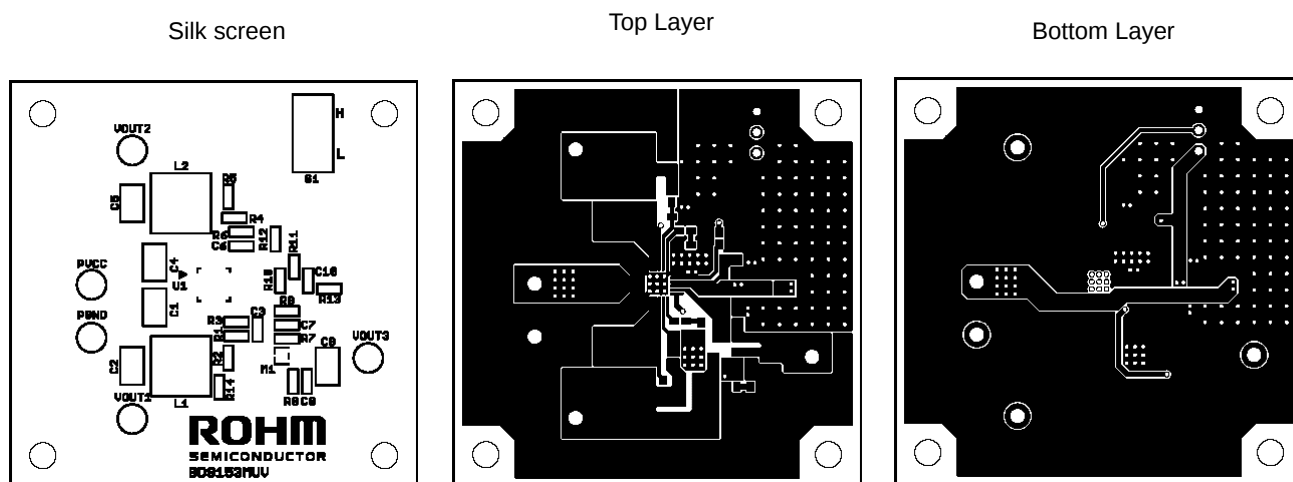
Fig.42 Layout diagram
