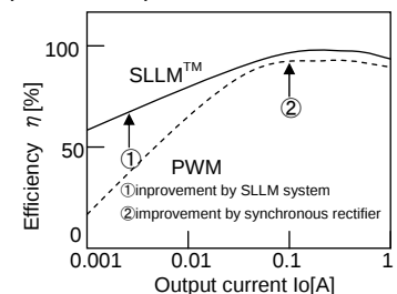
Fig.27 Efficiency
