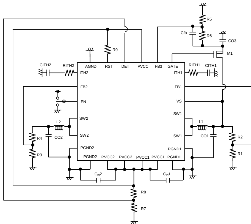
Fig.40 Typical application
