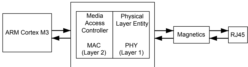
Figure 16-1. Ethernet Controller
