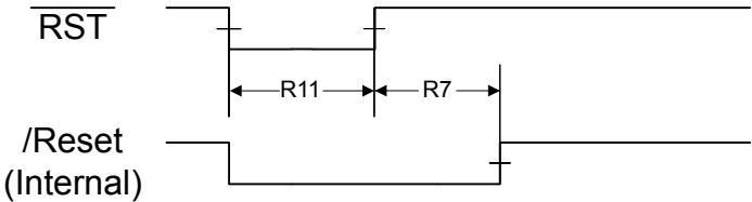
Figure 21-6. Power-On Reset Timing
