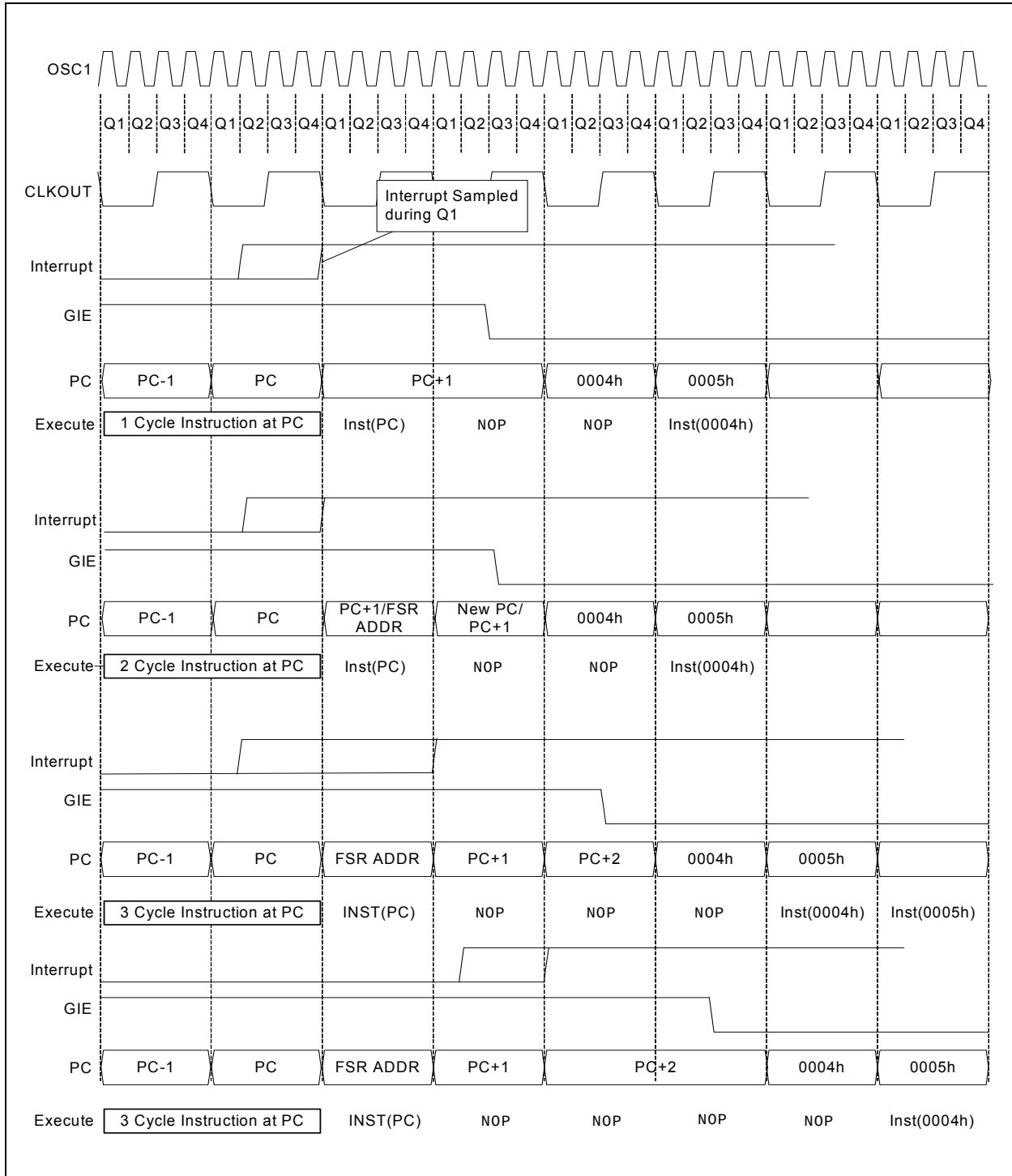
FIGURE 7-2: INTERRUPT LATENCY
