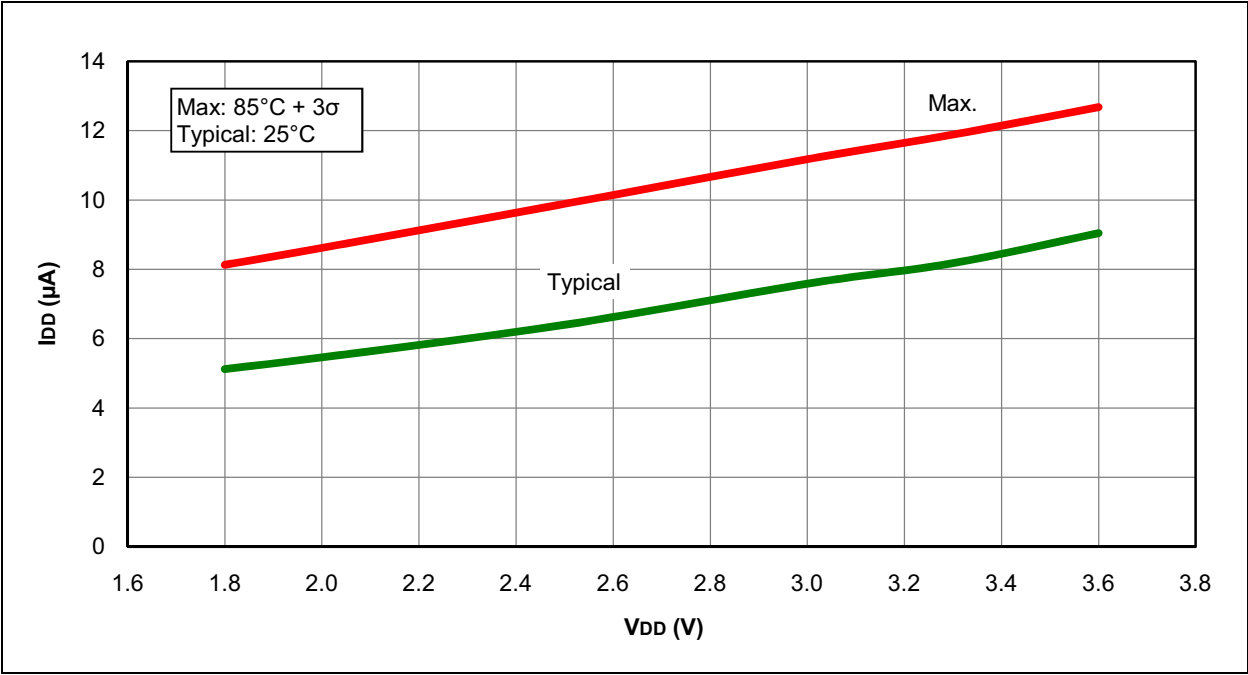
FIGURE 31-1: I_{DD} , LP OSCILLATOR MODE, F_{osc} = 32\text{ kHz} , PIC16LF1946/47 ONLY
