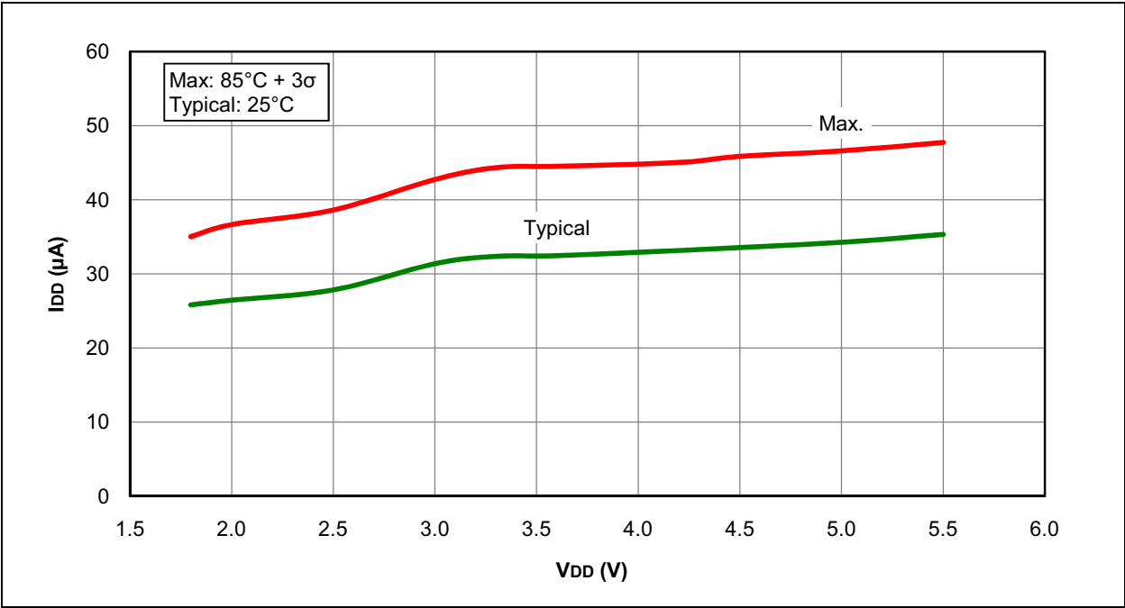
FIGURE 31-2: I_{DD} , LP OSCILLATOR MODE, F_{osc} = 32\text{ kHz} , PIC16F1946/47 ONLY
