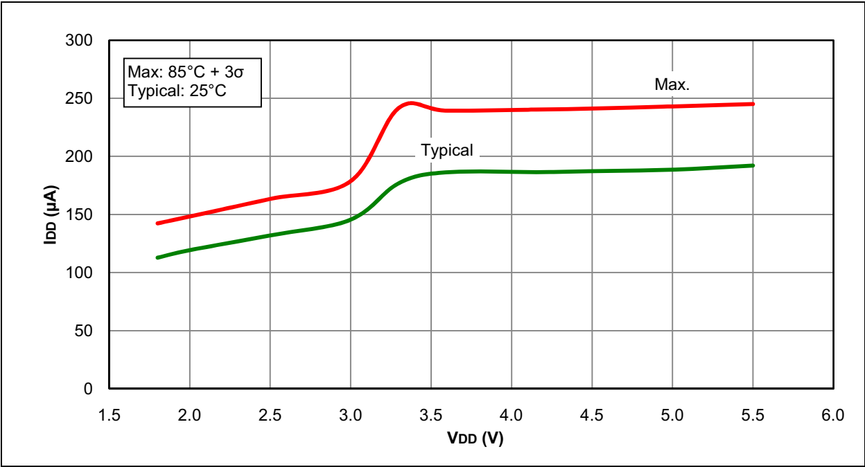
FIGURE 31-22: I_{DD} , MFINTOSC MODE, F_{osc} = 500\text{ kHz} , PIC16F1946/47 ONLY
