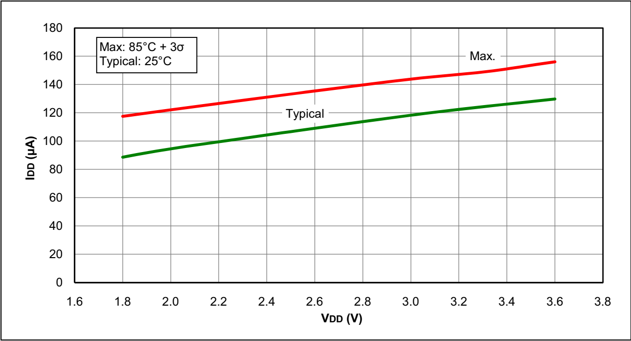
FIGURE 31-21: I_{DD} , MFINTOSC MODE, F_{osc} = 500\text{ kHz} , PIC16LF1946/47 ONLY
