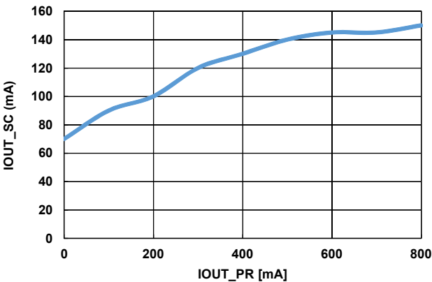
Figure 17. IOUT_SC± vs Corresponding IOUT_PR (VOUT = 12V)
